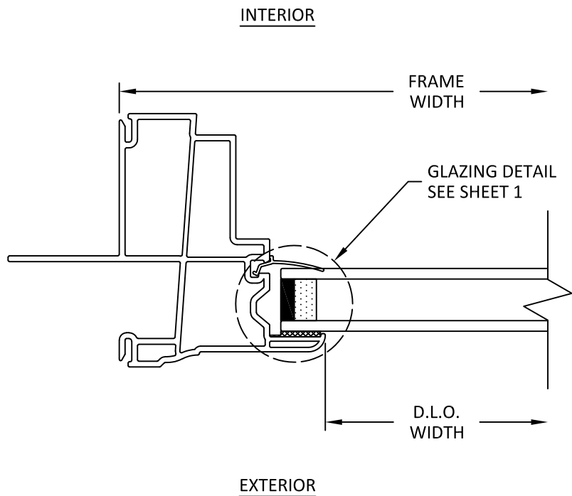
C 4 HORIZONTAL SECTION WINDOW JAMB
