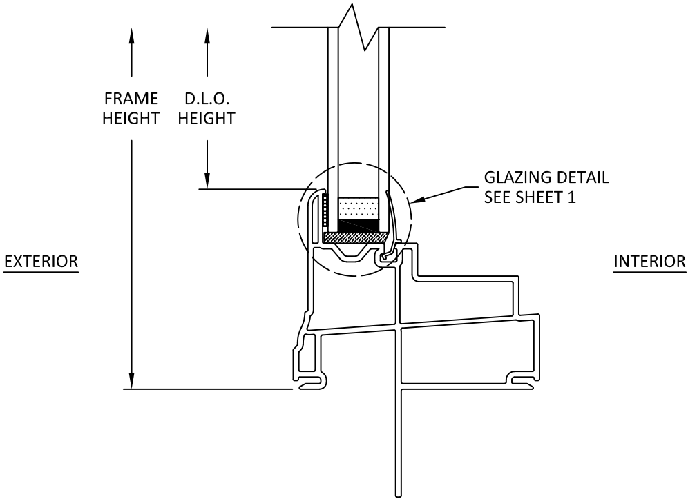
B 3 VERTICAL SECTION WINDOW SILL
