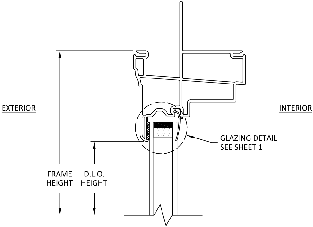
A 3 VERTICAL SECTION WINDOW HEAD
