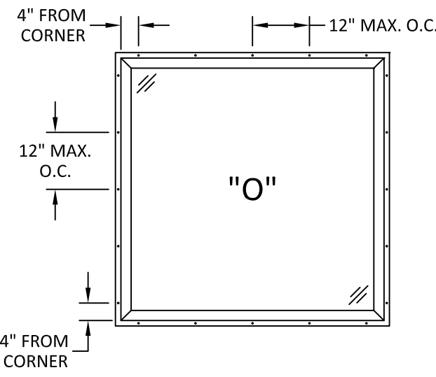
ANCHOR LAYOUT NAIL FIN
