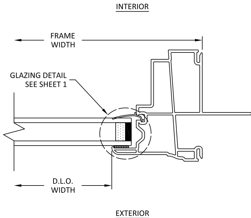
D 4 HORIZONTAL SECTION WINDOW JAMB
