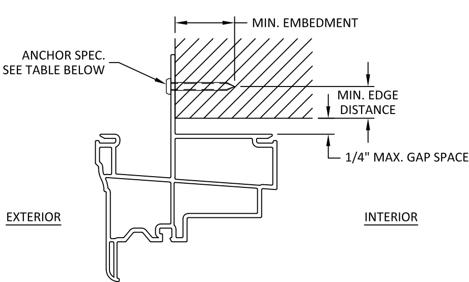
E 5 INSTALLATION DETAIL NAIL FIN HEAD INSTALLATION
